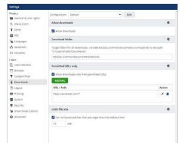
Fig. 7: Files & Downloads
