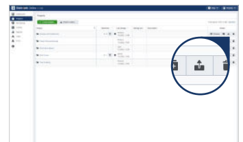
Fig. 2: Remote configuration
