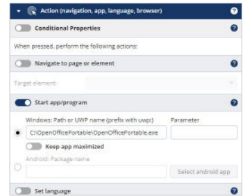
Fig. 6: Allowed applications
